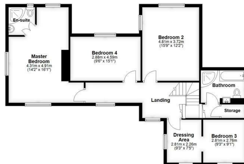
First Floor Approx. 96.3 sq. metres (1036.1 sq. feet)
